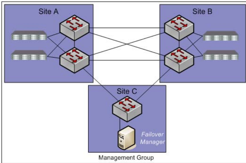
Figure 9 Hub and spoke network core with redundant links out to each site
