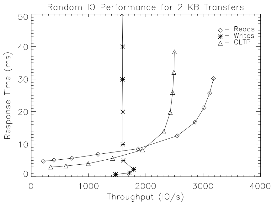
FIGURE 1. Random I/O performance for 2 KB transfers
