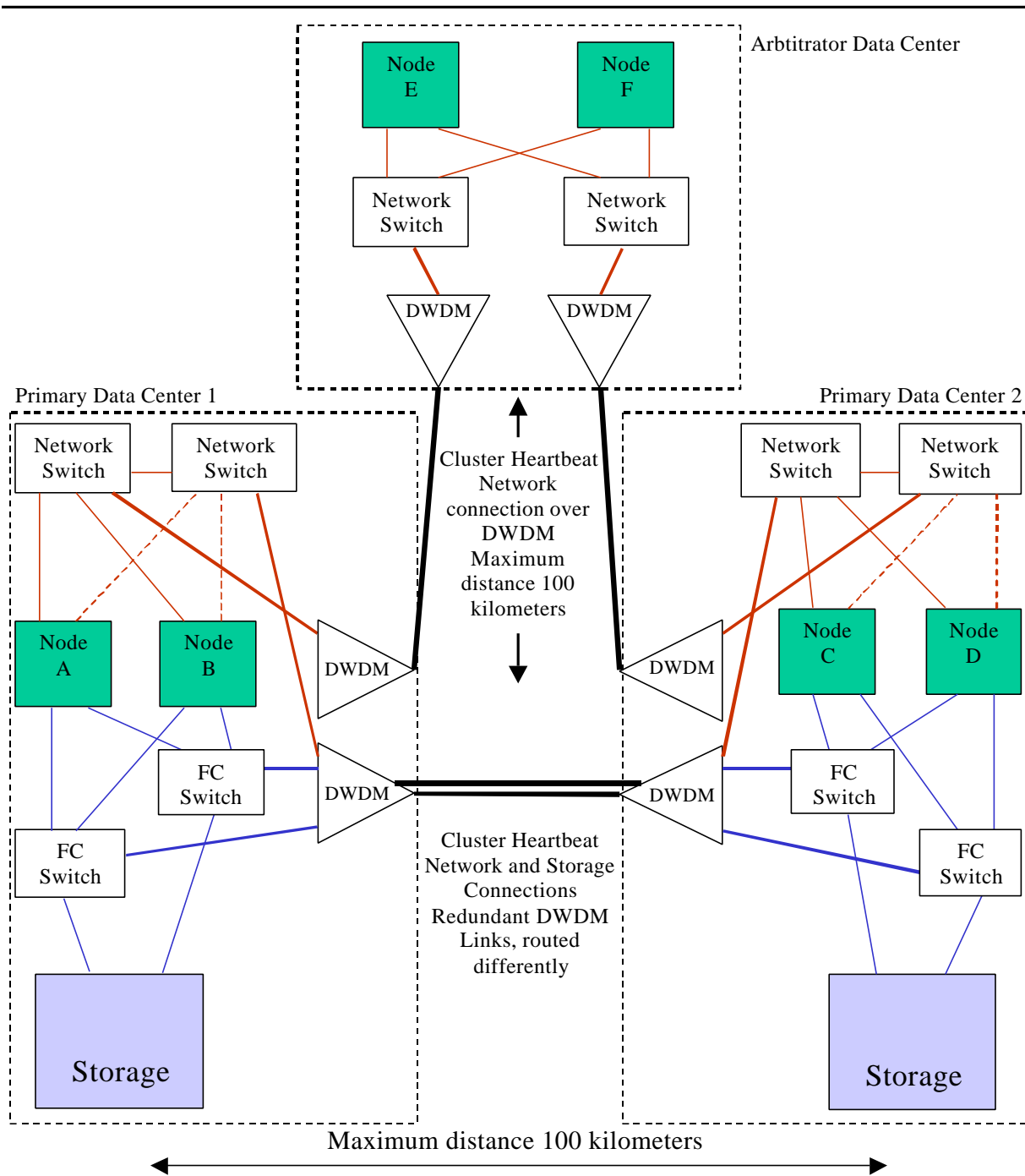
Figure 3 Extended MC/ServiceGuard cluster configuration with three data centers and DWDM
