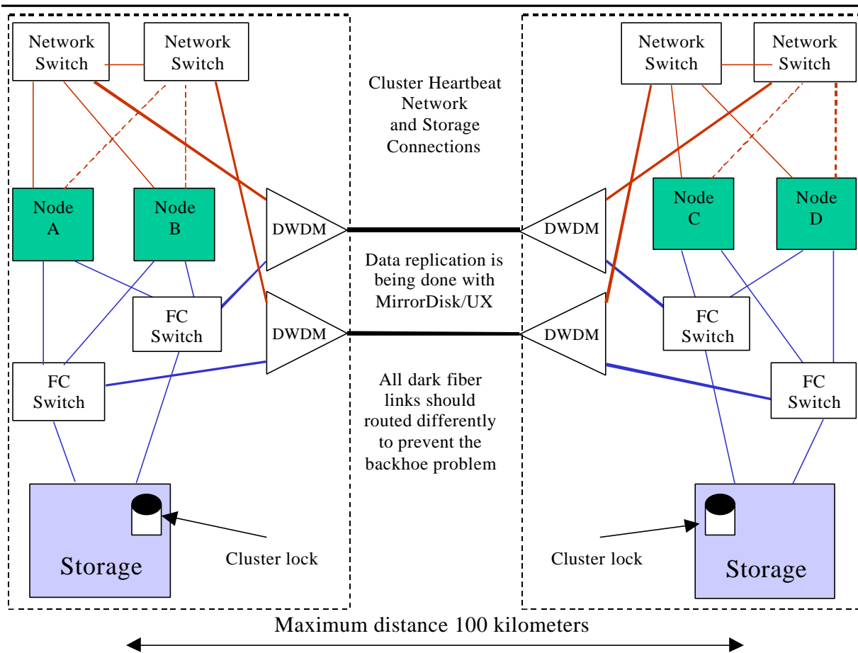
Figure 2 Extended MC/ServiceGuard cluster configuration with two data centers and DWDM
