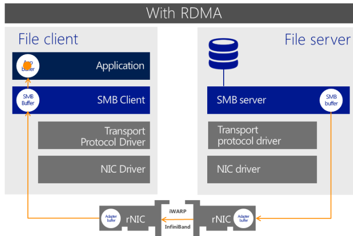
Figure 21: A client and server example with SMB Direct and RDMA.
