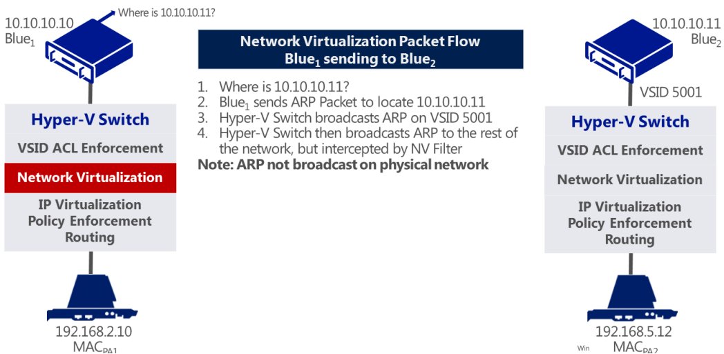
Figure 5: The Hyper-V Switch then broadcasts ARP to the rest of the network, but the packet is intercepted by NV Filter.
