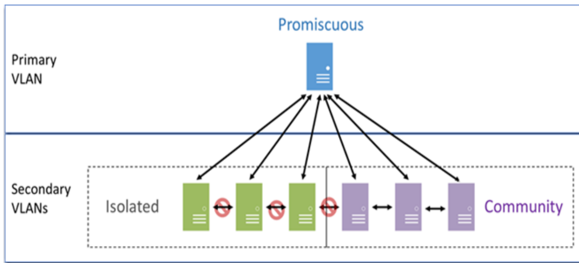
Figure 29: A PVLAN consists of a primary and secondary VLAN pair.
