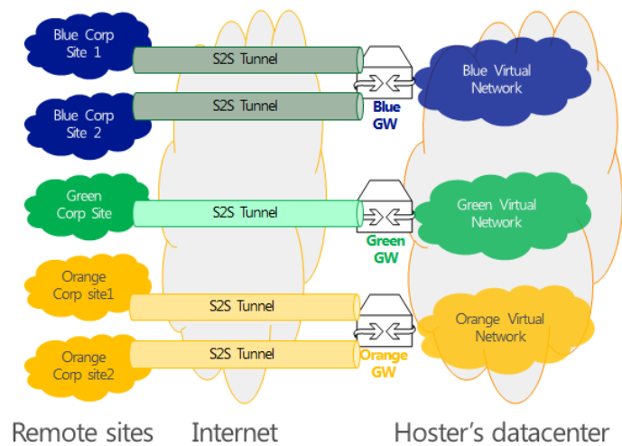
Figure 35: Hybrid networking in Windows Server 2012 R2.
