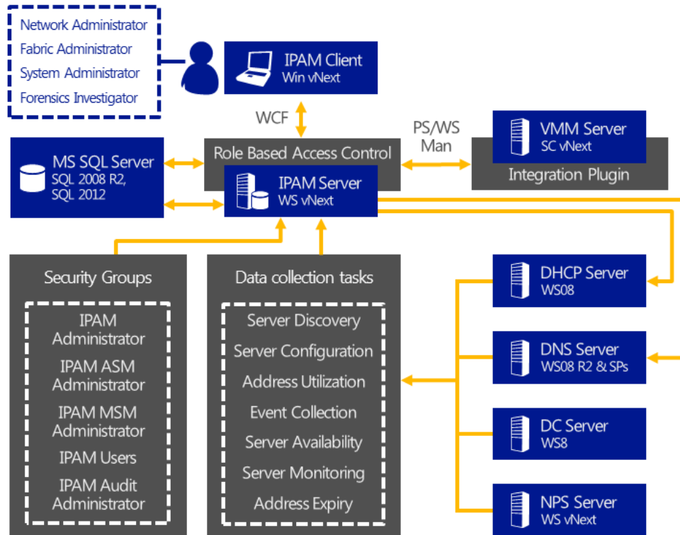
Figure 25: A centralized deployment of IPAM.
