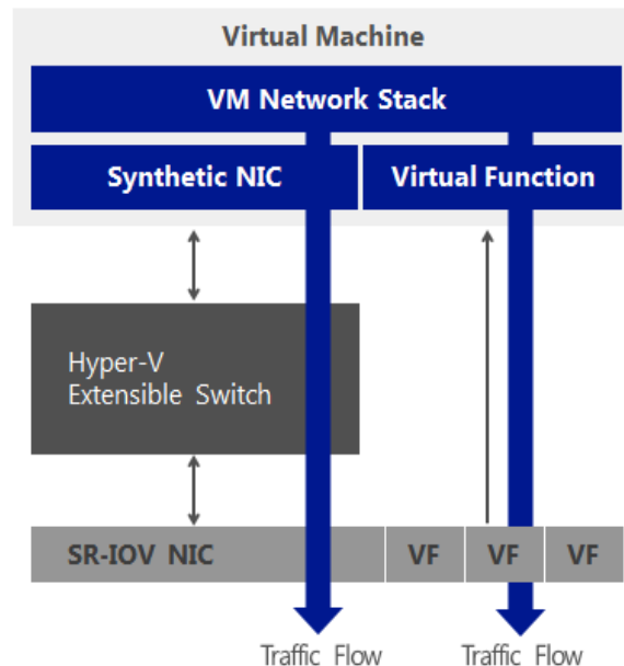
Figure 23: SR-IOV maps virtual network functions from the NIC directly to the virtual machine.
