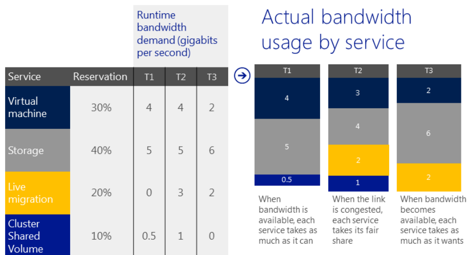
Figure 18: How relative minimum bandwidth works for different network flows.
