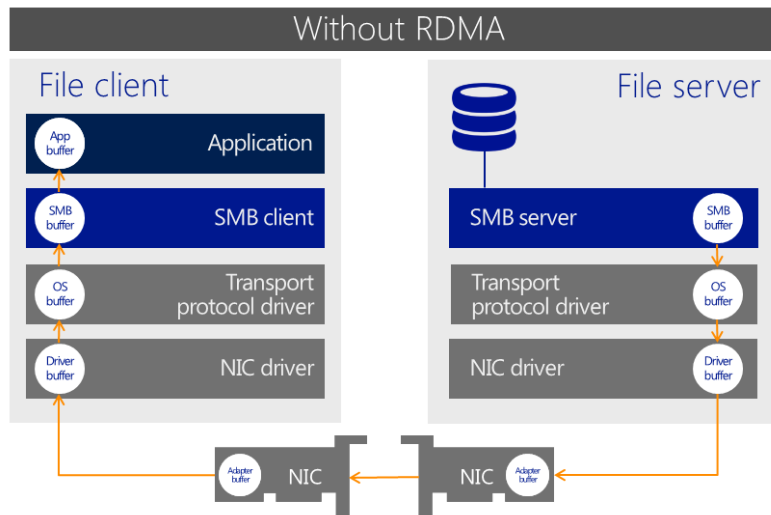
Figure 20: A client and server example without SMB Direct and RDMA.
