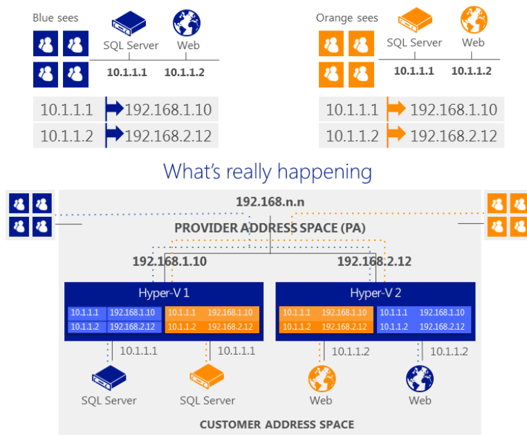
Figure 1: Using HNV to overlay two virtual networks over the same PA address space.
