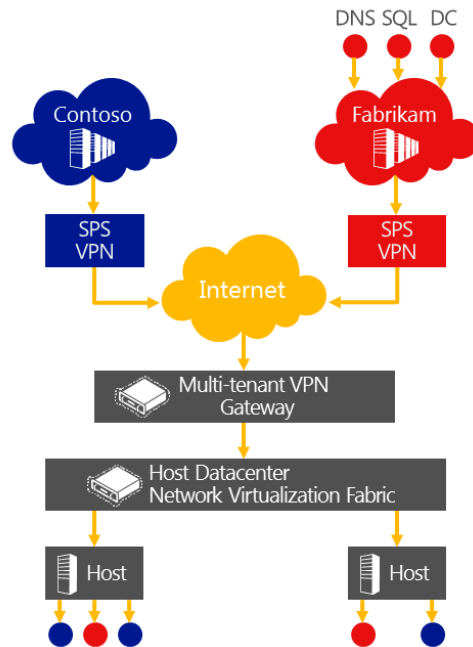
Figure 13: The Windows Server 2012 R2 Multi-Tenant VPN Gateway.
