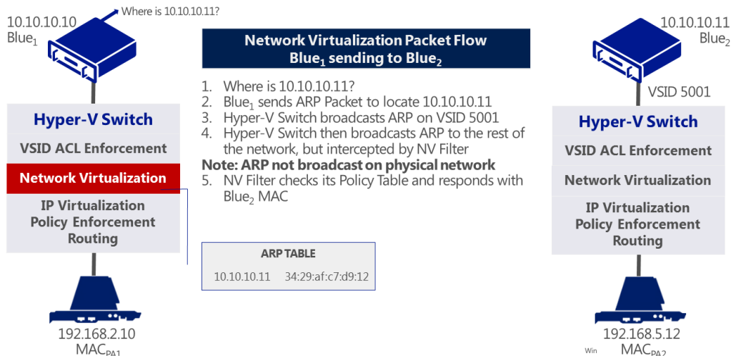
Figure 6: The NV Filter checks its Policy Table and responds with Blue2 MAC.
