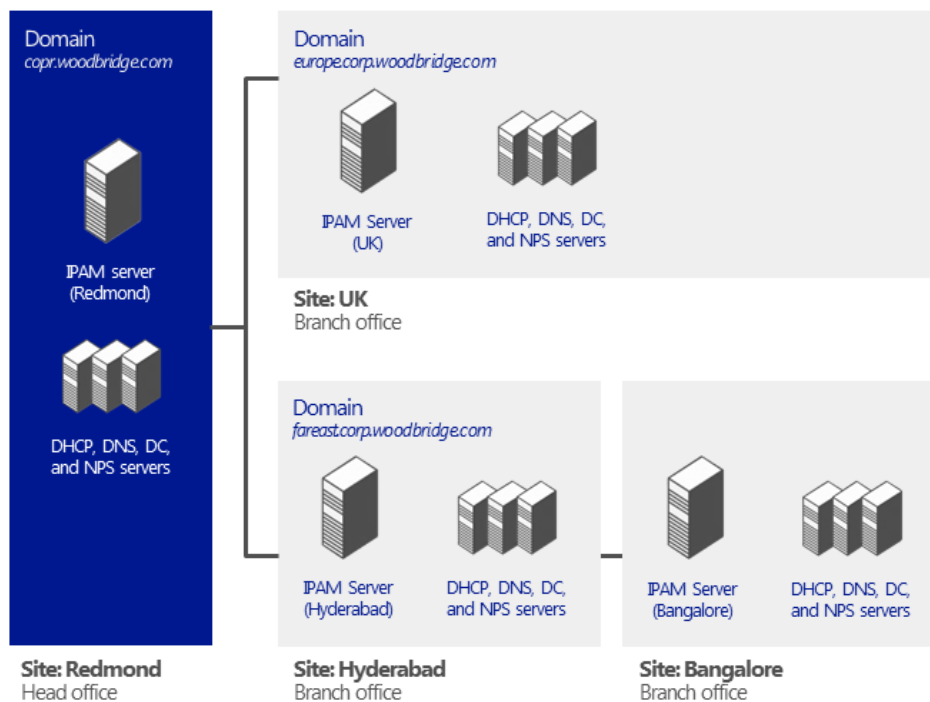
Figure 24: An IPAM-distributed architecture.
