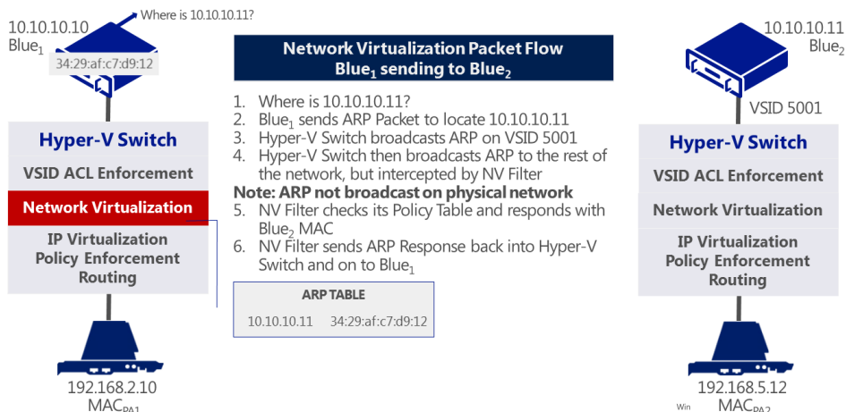
Figure 7: The NV Filter sends the ARP Response back into Hyper-V Switch and on to Blue1.
